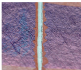
Destructive dry film thickness test
